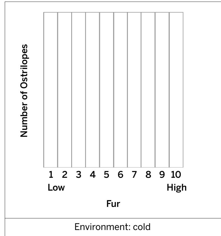
2. Population After 50 Generations
